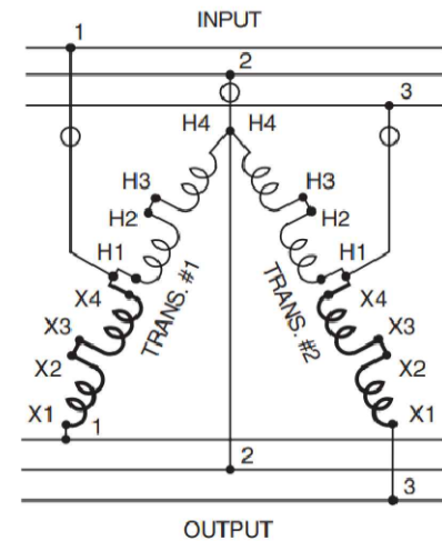
FIG. BB OPEN DELTA
