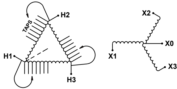
COIL TAP ARRANGEMENT
