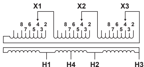
COIL TAP ARRANGEMENT
