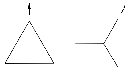
PHASOR DIAGRAM
