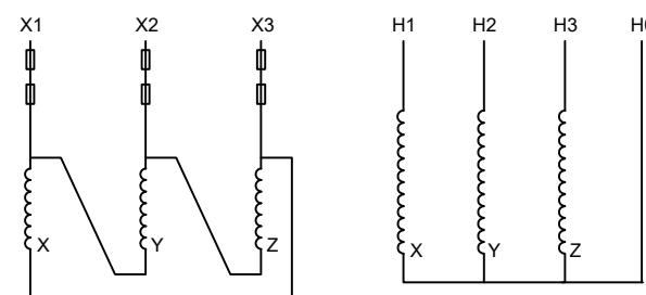
WIRING CONNECTION
