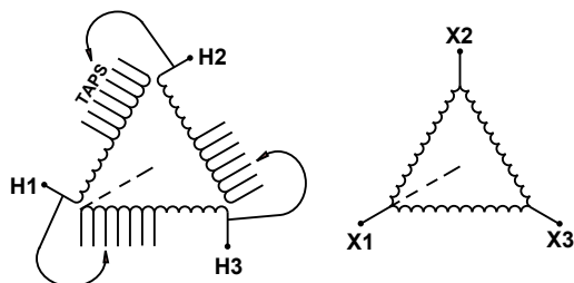
COIL TAP ARRANGEMENT
