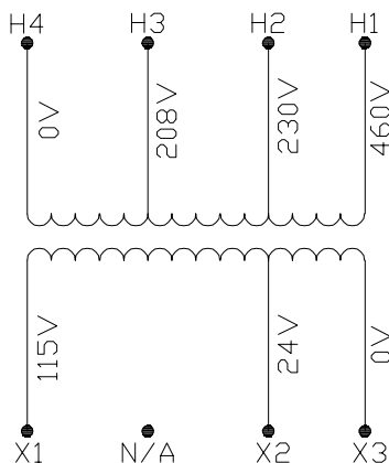
CONNECTION DIAGRAM
