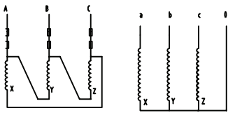
WIRING CONNECTION
