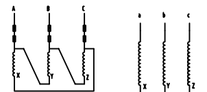
WIRE CONNECTION
