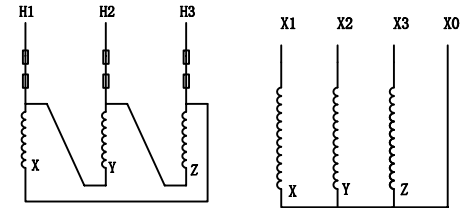
WIRING CONNECTION
