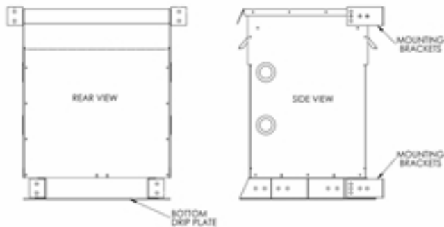
Image: MT-XX-DTM-WM-30KVA
