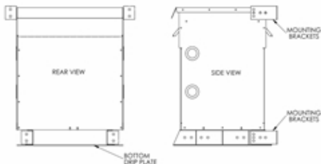
Image: MT-XX-DTM-WM-75KVA
