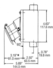
* Malleable iron receptacle: 3.38"/85.6 mm
