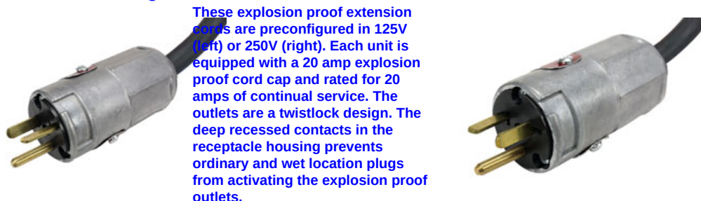
125V 5-20P Explosion Proof Straight Blade Plug
