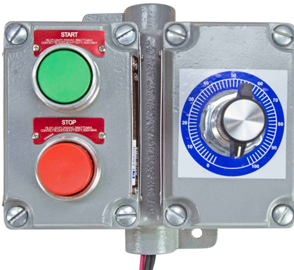
Image: EPCS-2XPB.MS-24V-PTM.5K-25FT
