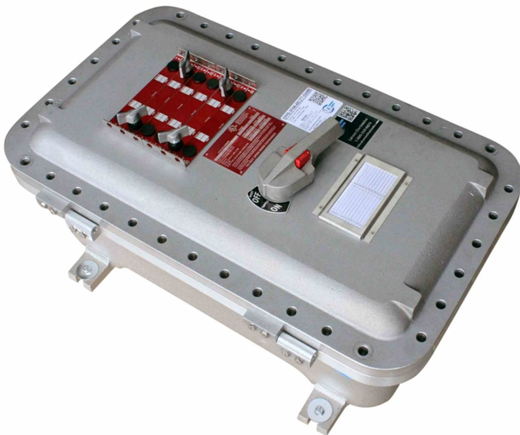
Image: EPPB-3P4W-480Y.277-100AMB-2X40.2-1X20.2-10X20.1
