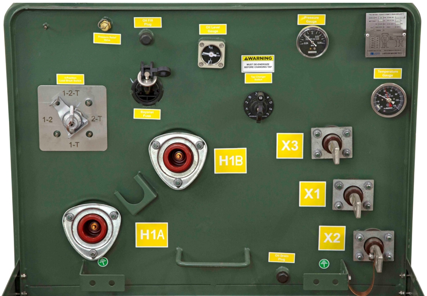
Image: MT-PML-R7-3P-DVD-112.5KVA-YE-LT-DF-A6-BB-CZ-2B4-M1
