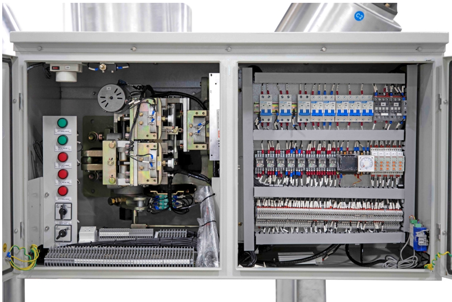
Image: MT-DTCB-SF6-R7-3P-AC-DXK-1200A-63KA-6-FM-Z-Z-N4X-M3
