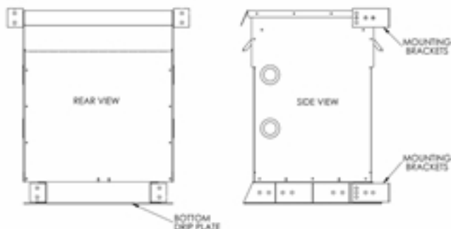
Image: MT-XX-DTM-WM-30KVA
