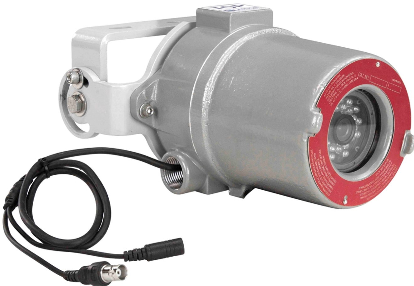
Image: EXPCMR-ALG-HDSD-1080P-12VDC
