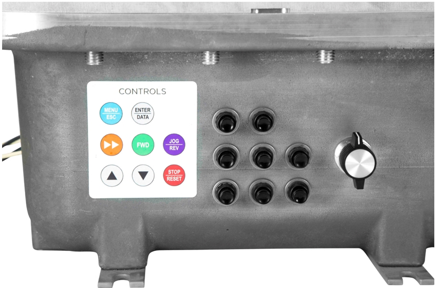
Image: EXP-VFD-1P-110.120-0.5HP-10A-DCM
