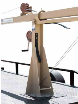
Manual 1,000 lb hand crank winch for elevating and folding over the light mast on the LM-30-3S-TLR10-JB.
