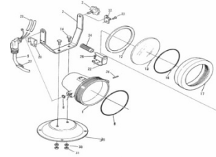
EPL-BS-70LED-100X12 Exploded View
