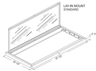
HAL-LI-48-2L-LED Dimensions
