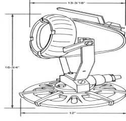
EPL-PM-1X30LED-120X12I-100
