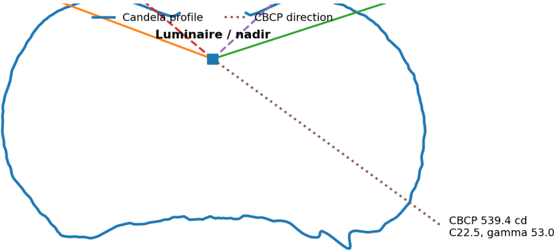
Beam Angle Diagram - Thresholds Referenced to Global CBCP
