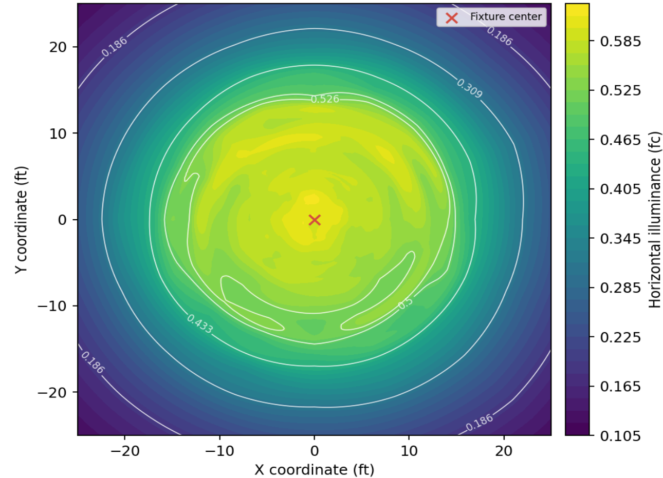
Iso-Foot-Candle Contour Map - 20 ft Mounting Height, LLF 0.80
