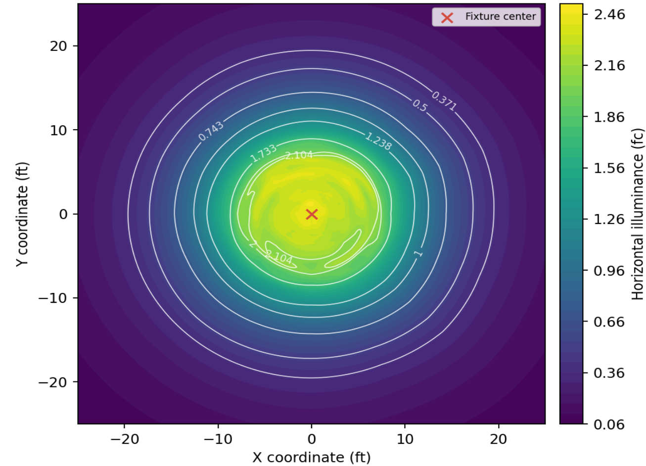
Iso-Foot-Candle Contour Map - 10 ft Mounting Height, LLF 0.80
