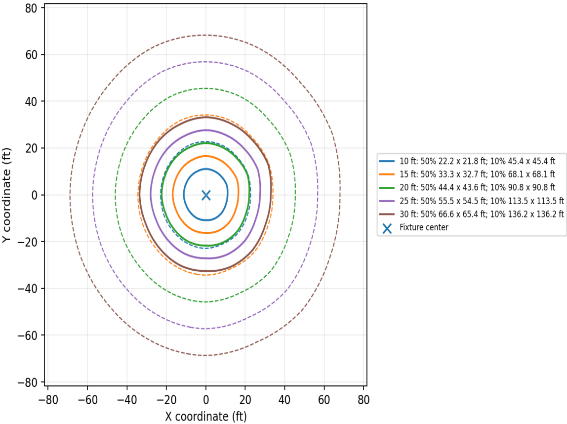
Top-View Practical Beam Footprints at Requested Mounting Heights
