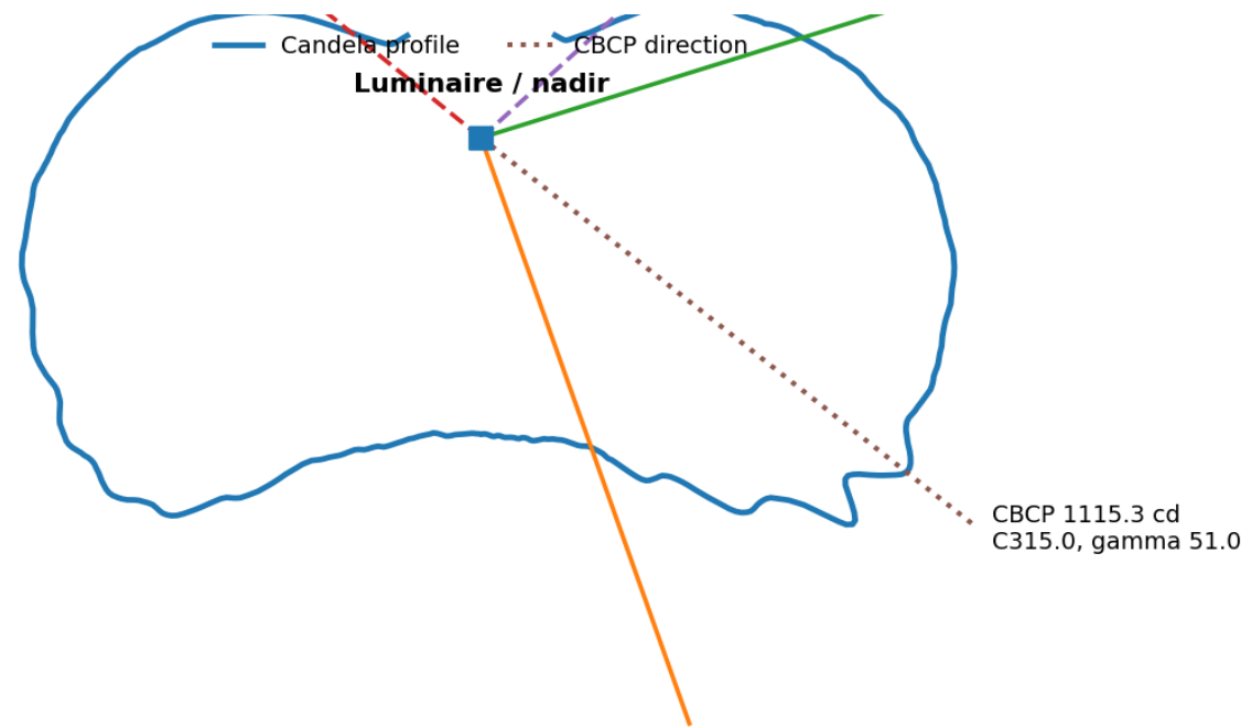
Beam Angle Diagram - Thresholds Referenced to Global CBCP
