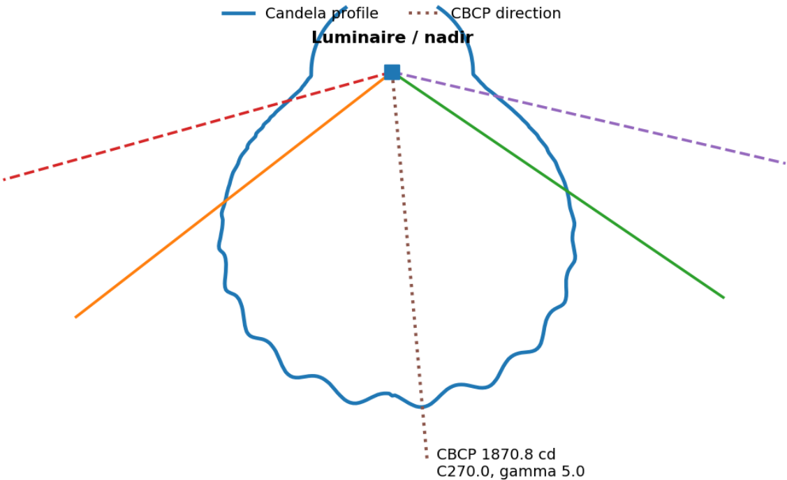
Beam Angle Diagram - Thresholds Referenced to Global CBCP
