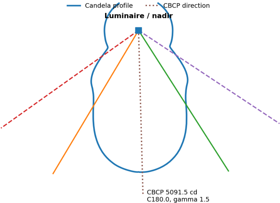
Beam Angle Diagram - Thresholds Referenced to Global CBCP
