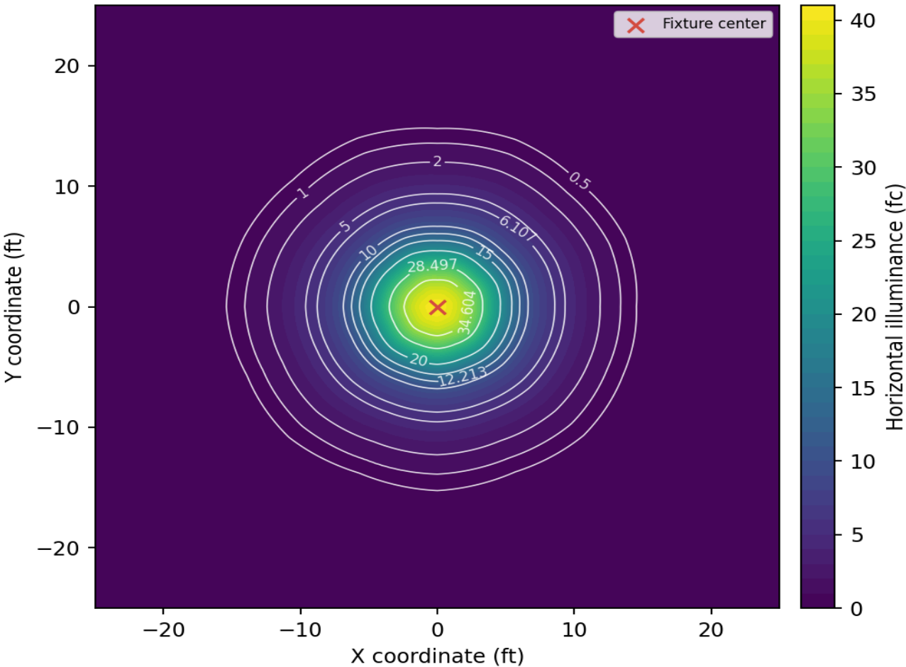
Iso-Foot-Candle Contour Map - 10 ft Mounting Height, LLF 0.80
