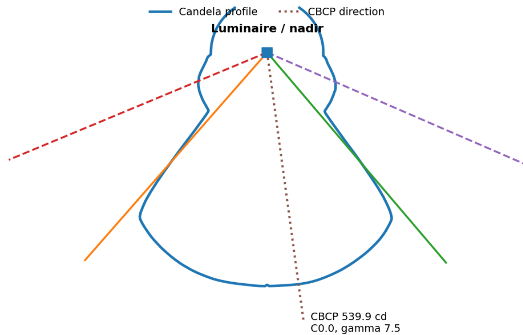
Beam Angle Diagram - Thresholds Referenced to Global CBCP
