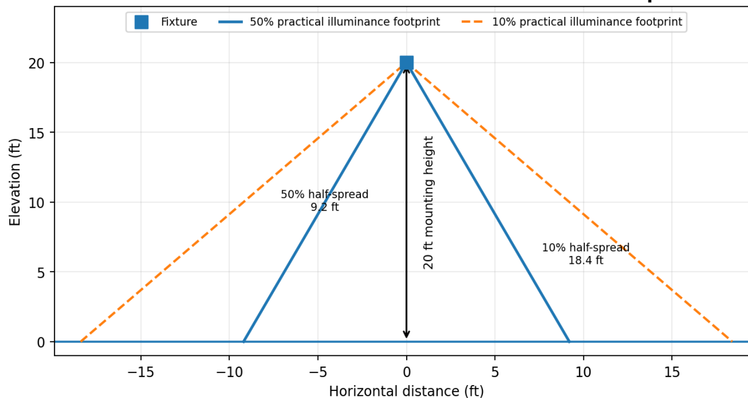
Side-View Beam Profile - Practical Ground-Plane Footprint
