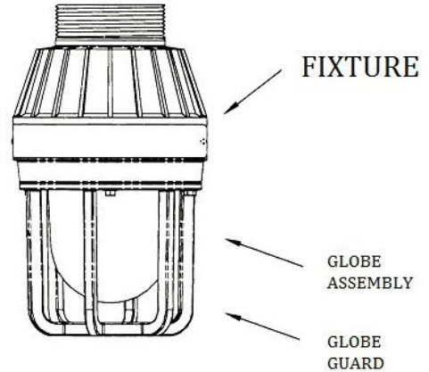
COMPONENT DRAWING
