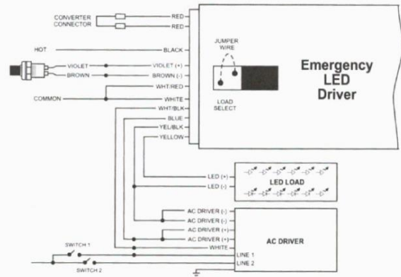
FIG B STEP DIMMING INSTALLATION
