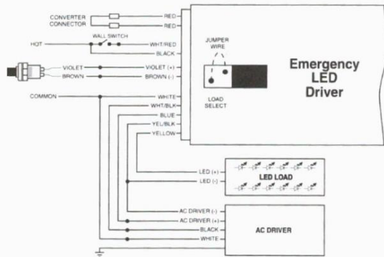
FIG A TWO (2) WIRE INTEGRATED TEST SWITCH
