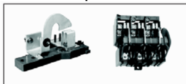
FIG. 3 : Examples of Line Base Assemblies
