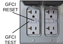
20A 120V AC 5-20R GFCI
