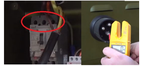
Testing Continuity between main breaker and plug.
