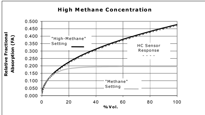
Figure 6. Comparison of "Methane" to "High-Methane" linearization for high concentrations.
