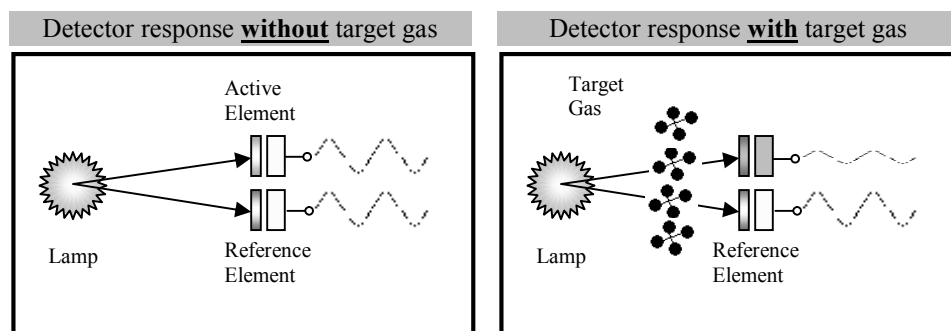
Figure 3. Signal outputs with and without gas exposure.
