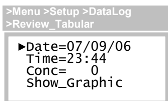
Figure 54. Data log tabular report page
