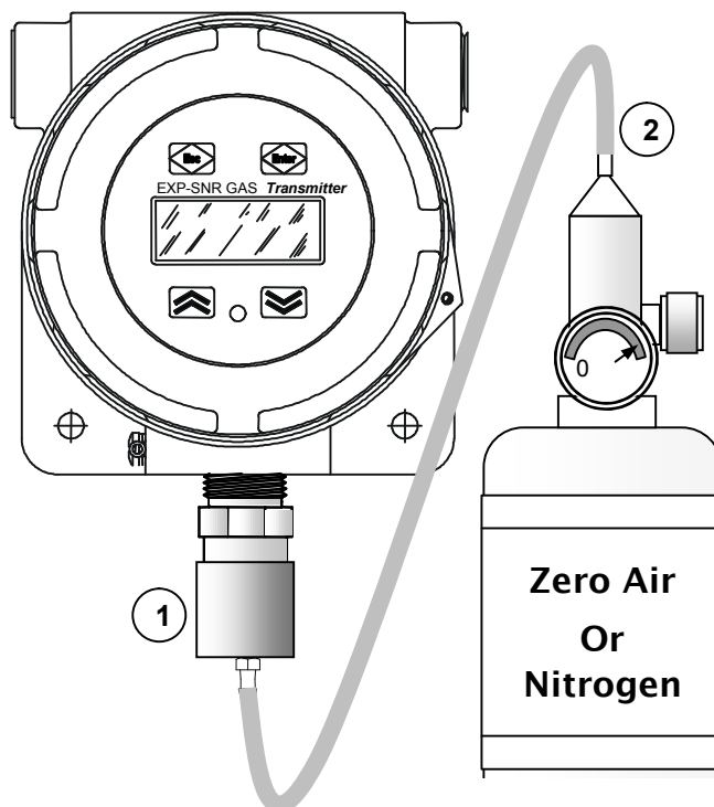
Figure 30. Zero calibration
