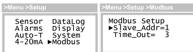
Figure 65. Modbus setup page
