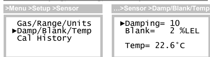
Figure 28. Sensor setup and Damp/Blank/Temp setup page
