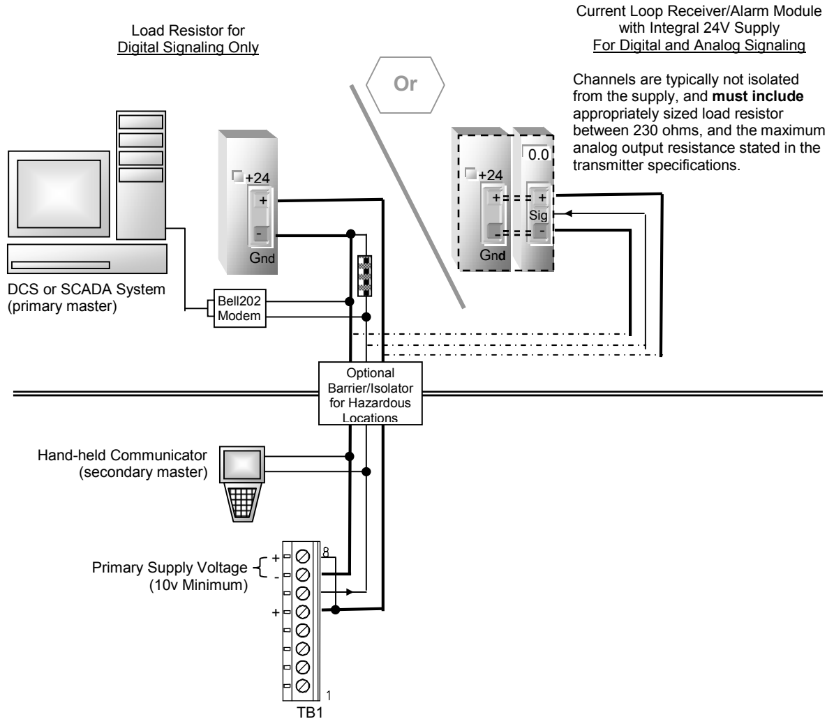
Figure 15. HART Transmitter, Point-to-Point, 3-Wire Example
