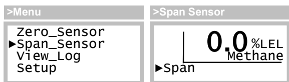
Figure 33. Span Sensor page
