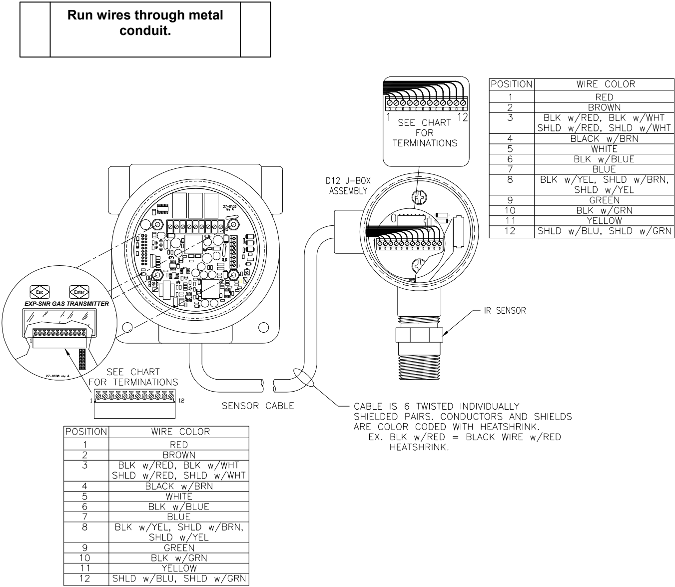
Figure 19. Remote Sensor Option wiring
