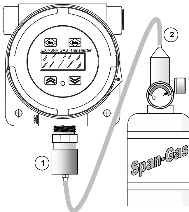
Figure 32 Span calibration
