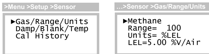
Figure 26. Sensor setup and Gas/Range/Units pages
