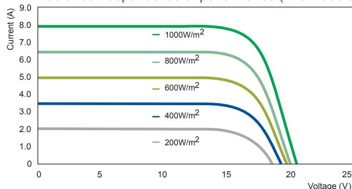
Irradiance - dependence of performance (140 module)
