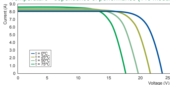
Temperature - dependence of performance (140 module)
