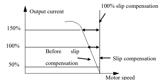
Fig.6-13 slip freq. compensation
