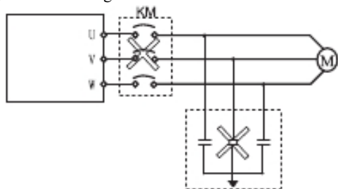
Fig. 1-3 Capacitor connection with VFD output prohibited
