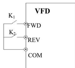
Fig.6-22 2-wire control mode1
