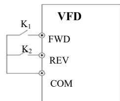
Fig.6-21 2-wire control mode1
