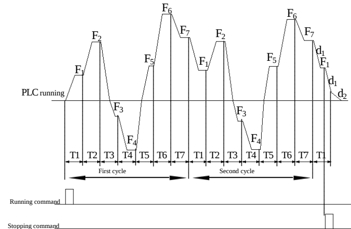
Fig.6-42 PLC continuous cycle
