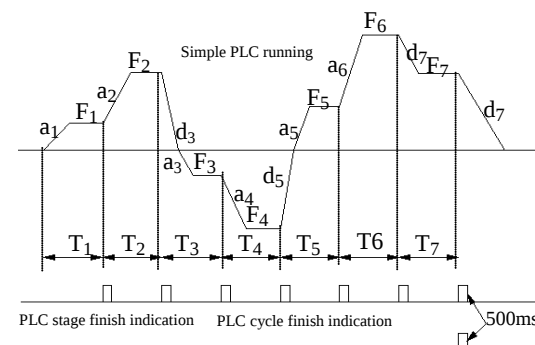
Fig.6-39 simple PLC running
