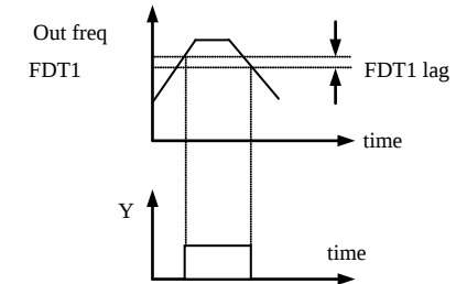
Fig. 6-27 freq level detection
