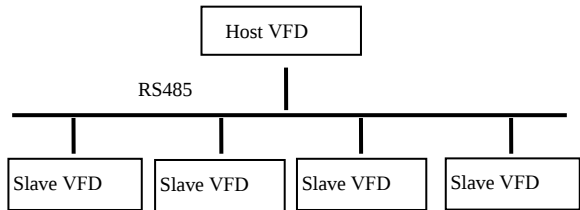
Fig. 9-2 The networking of multi-machine interaction
