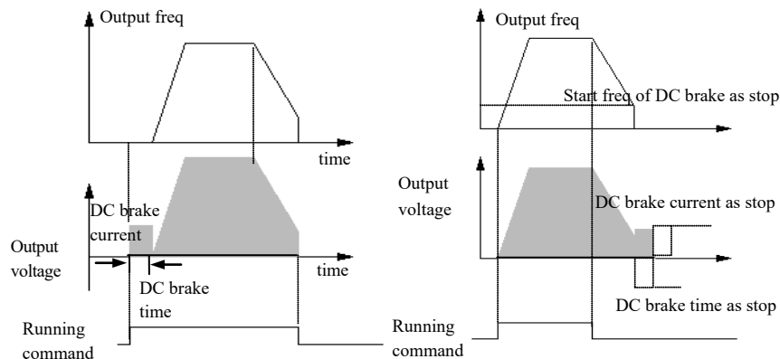
Fig.6-11 start mode 1
