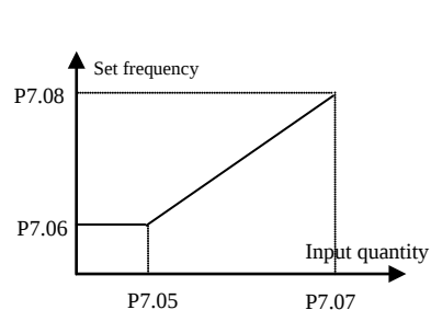
Fig.6-35 Inflection point invalid when the frequency setting of the 1
