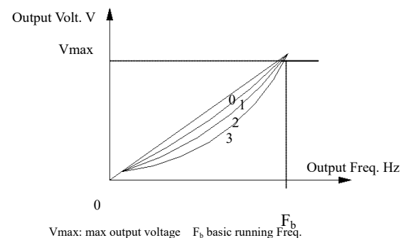
Fig. 6-7 V/F curve
