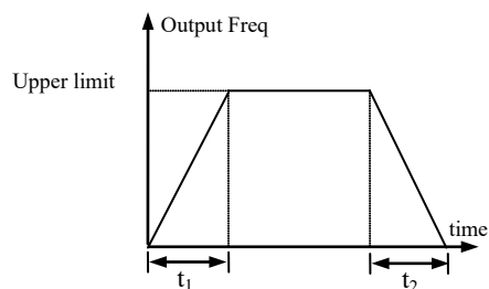
Fig.6-6 Acc/Dec time
