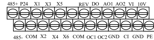
Fig. 3-7 CN2 terminals
