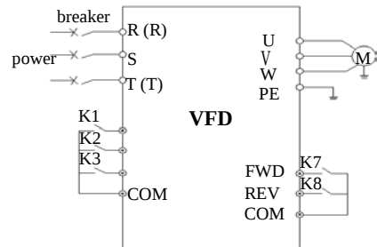
Fig.6-19 wiring diagram of multi-stage speed running
