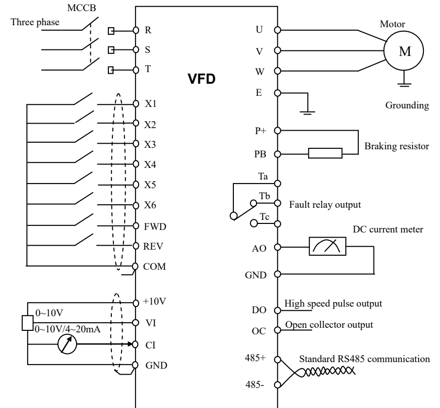
Fig. 3-5 Basic wiring diagram
