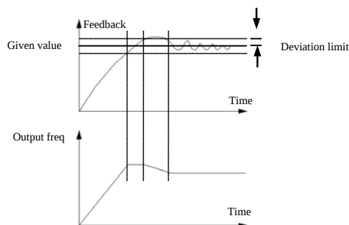
Fig.6-33 Deviation
