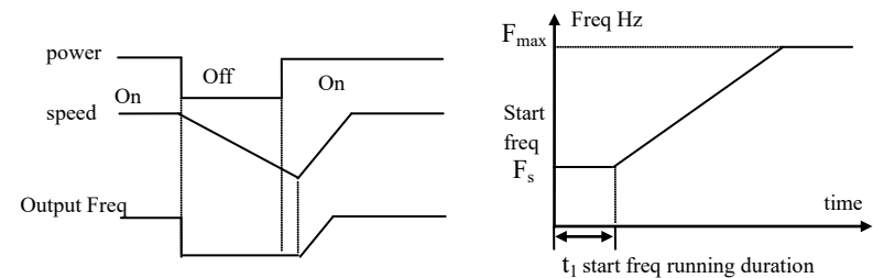
Fig.6-9 Speed tracking restart
