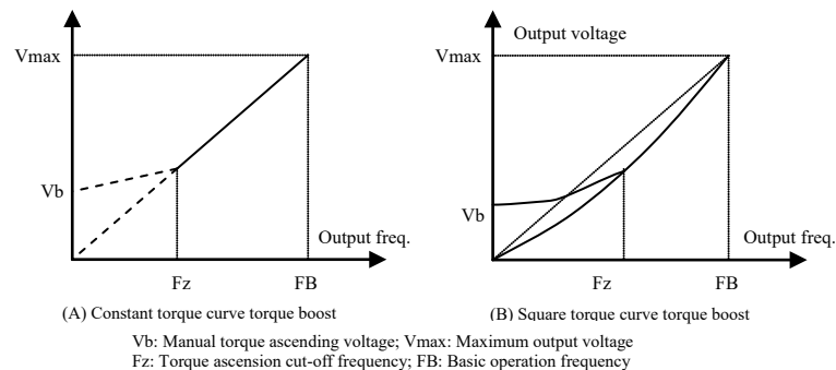
Fig.6-3 Torque boost
