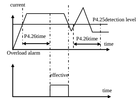
Fig. 6-29 overload alarm
