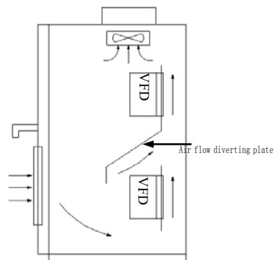
Fig. 3-2 Mounting of multiple VFDs
