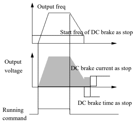
fig.6-12 DC stop and DC brake
