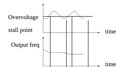
Fig.6-31 overvoltage stall
