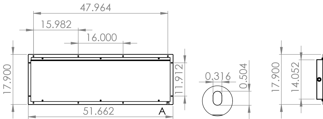
DETAIL A SCALE 1 : 2
