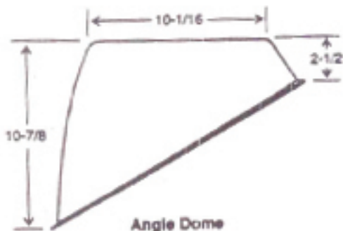
Angle Dome
