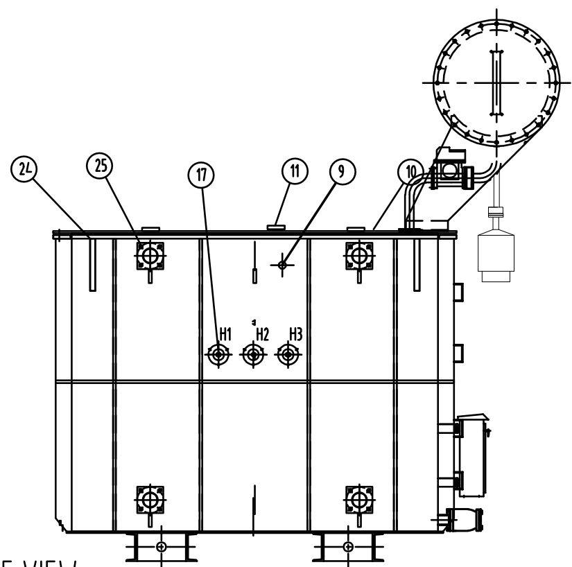
HV SIDE VIEW
