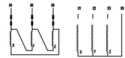
WIRING CONNECTION
