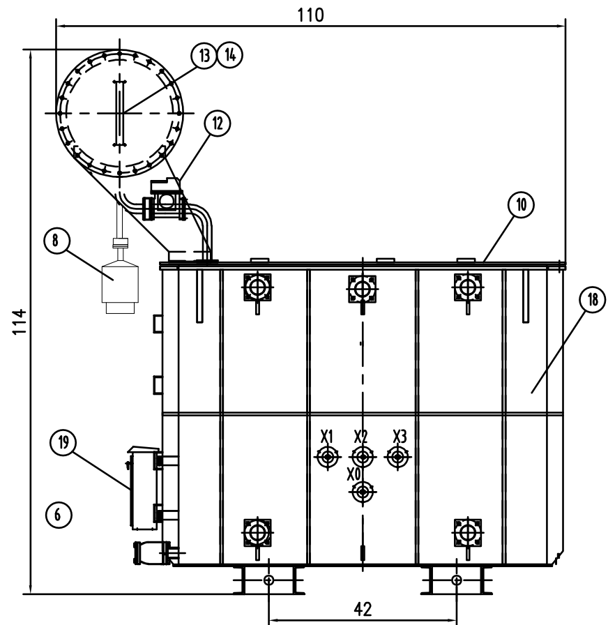
LV SIDE VIEW
