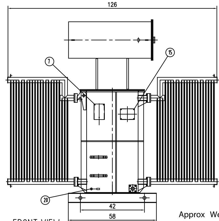
FRONT VIEW
