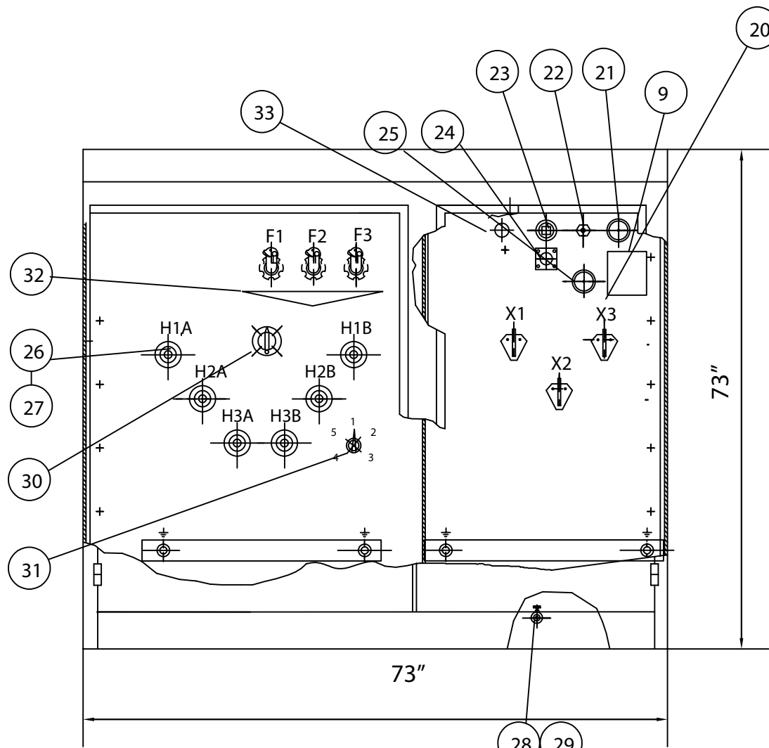
FRONT VIEW
