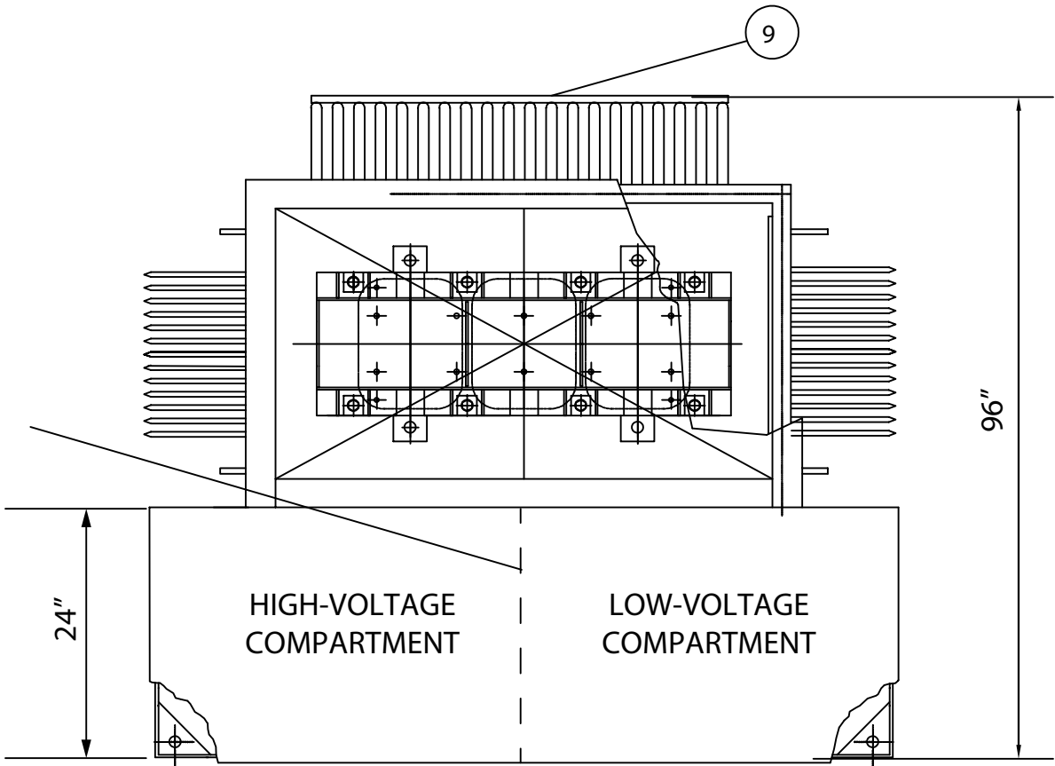
PAD VIEW
