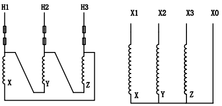
WIRING CONNECTION
