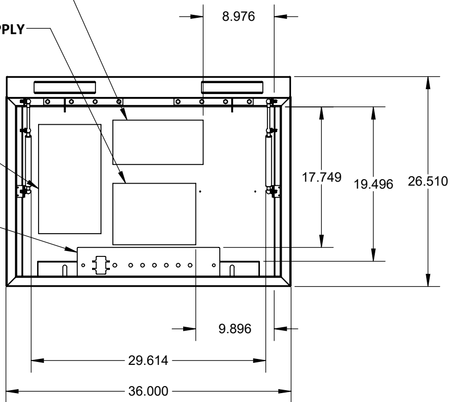
TOP VIEW
