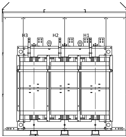
ANTI-VIBRATION PADS (6x) FRONT VIEW
