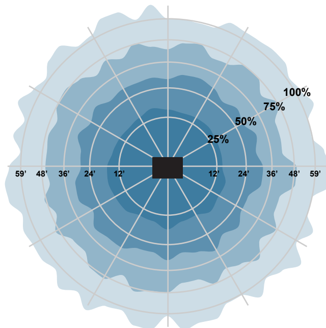
Ceiling Mounting Pattern
