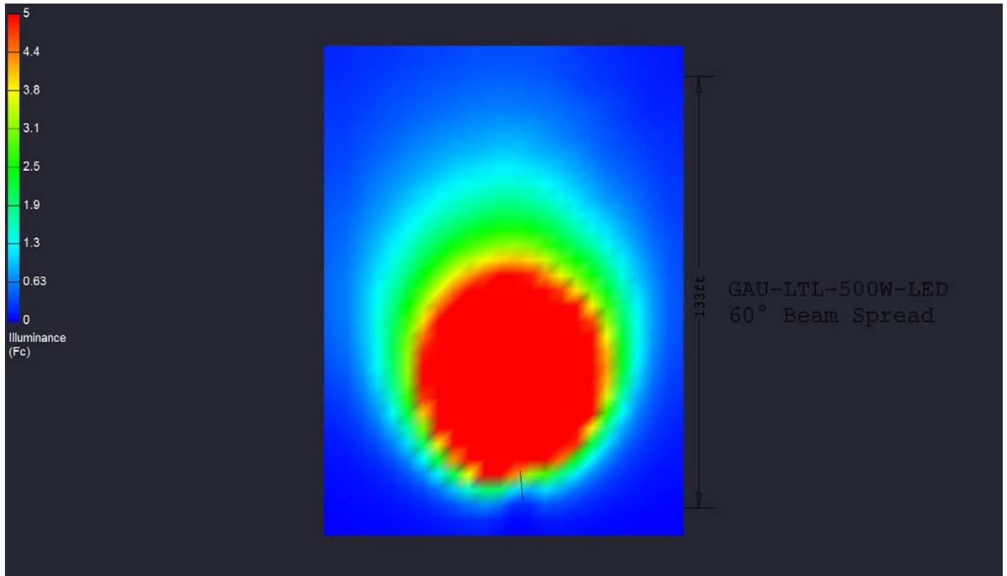
GAU-LTL-500W-LED 60 Degree
