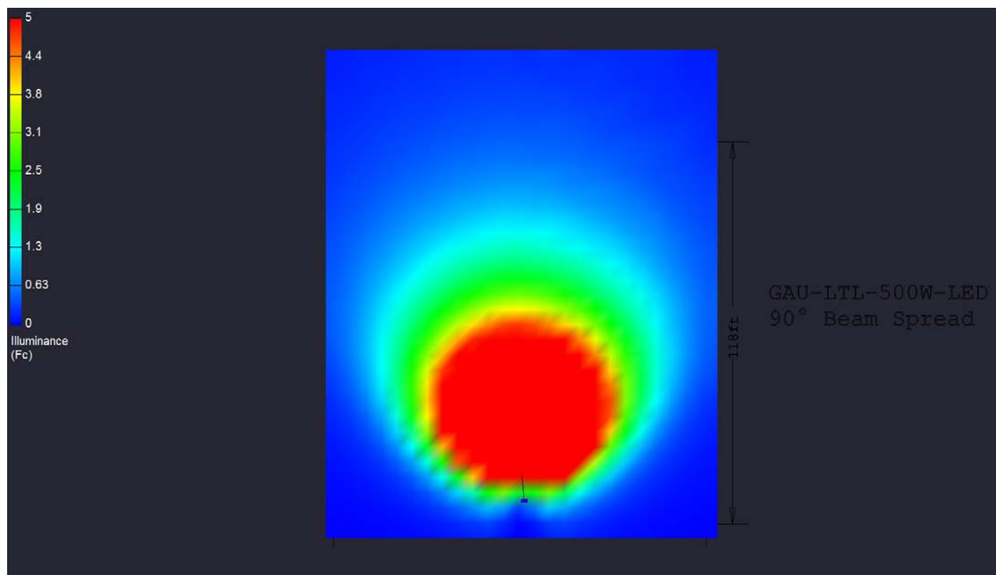
GAU-LTL-500W-LED 90 Degree
