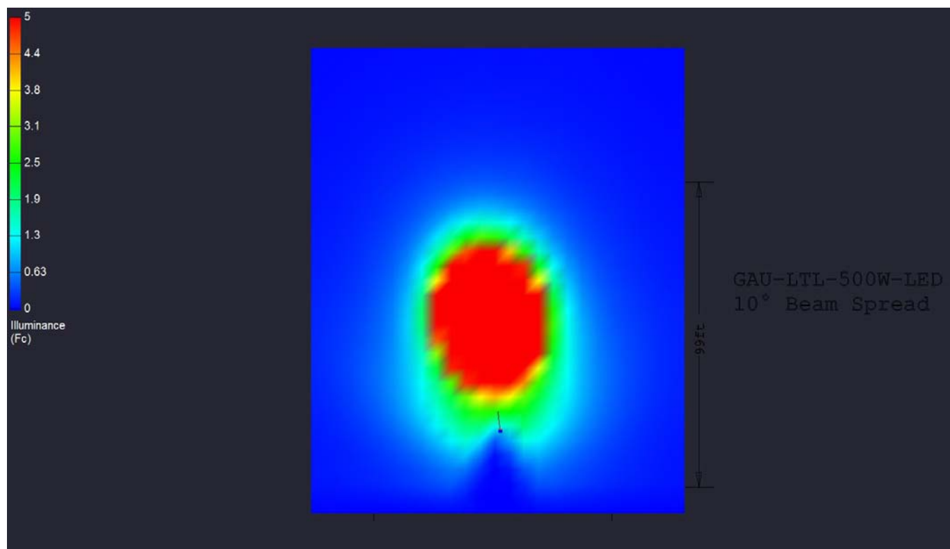
GAU-LTL-500W-LED 10 Degree
