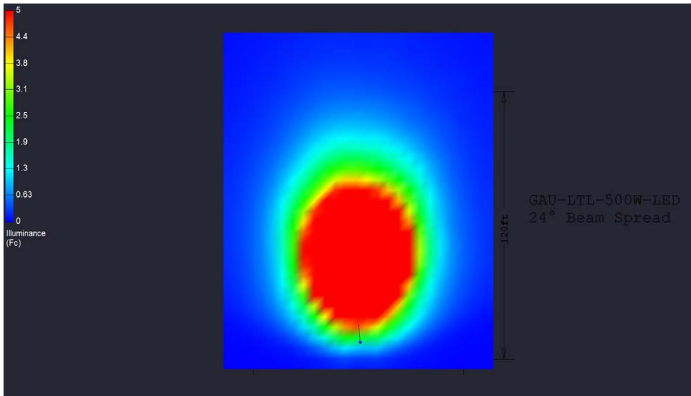
GAU-LTL-500W-LED 24 Degree
