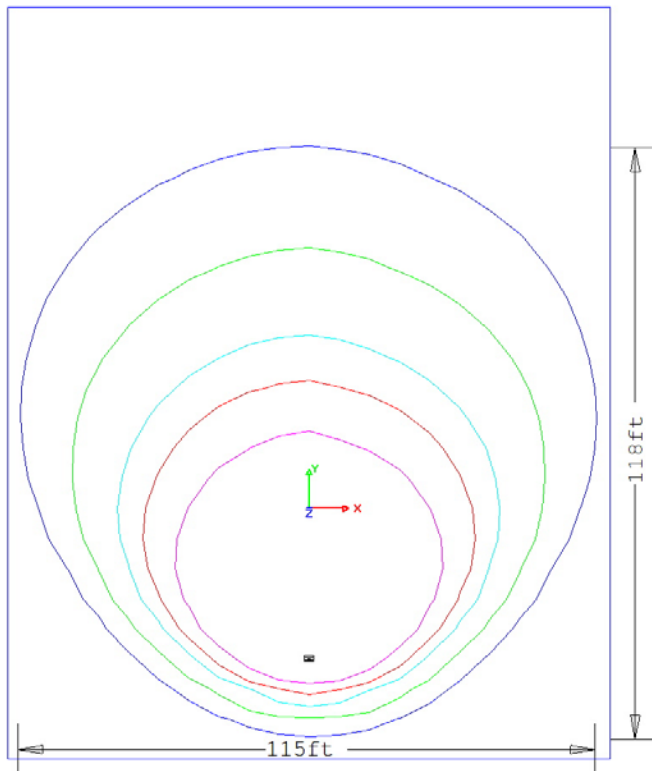
GAU-LTL-500W-LED 90° Beam Spread
